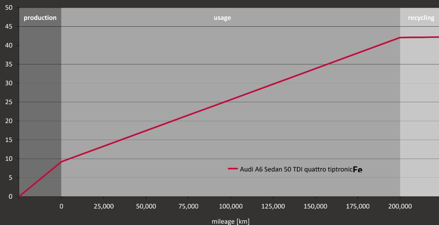
Figure 2: Global warming potential of the Audi A6 Sedan 50 TDI quattro tiptronic* over the entire life cycle
